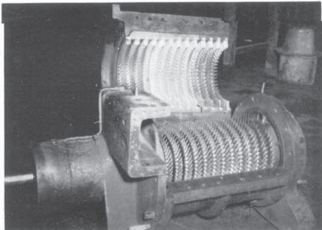
AXIAL FLOW COMPRESSOR
