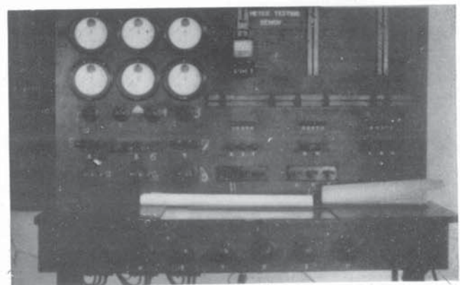
METER TESTING BENCH
