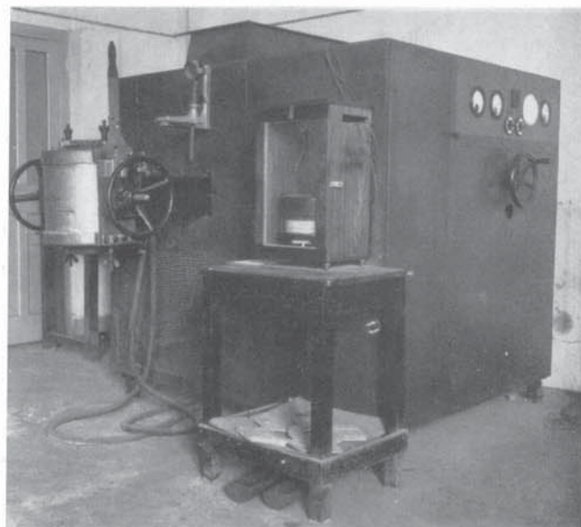
GRAPHITE RESISTANCE TYPE STEEL MELTING UNIT
