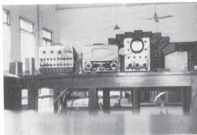
AN ELECTRICAL RESISTANCE STRAIN MEASURING EQUIPMENT—DYNAMIC STRAIN
