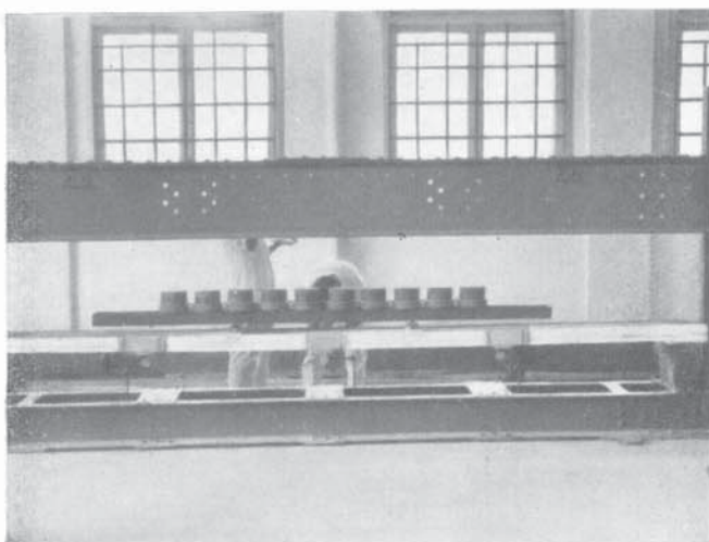
TESTING PRE-STRESSED CONCRETE FLOOR BEAM
