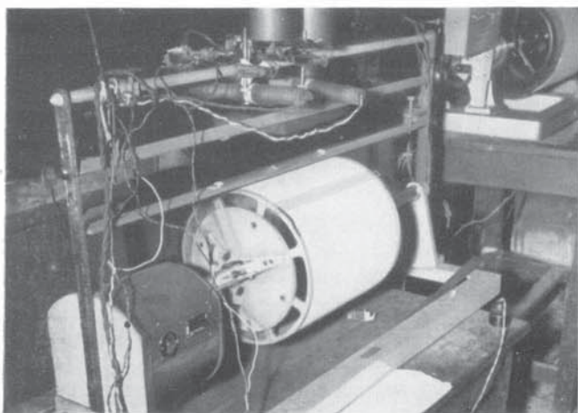
HIGH SPEED RECORDER FOR MICROSEISMS IN CYCLONIC DISTURBANCES
