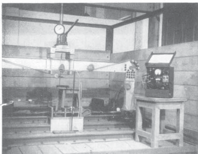
EXPERIMENTAL SET-UP FOR A PRE-STRESSED STEEL PORTAL
