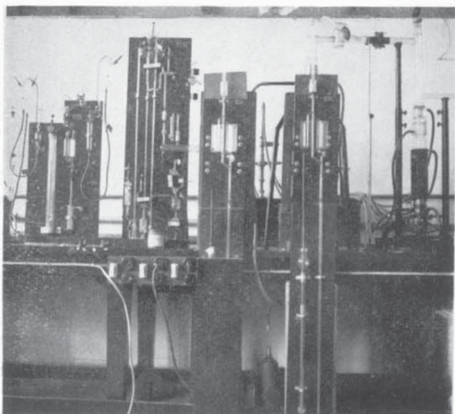
VACUUM FUSION APPARATUS
