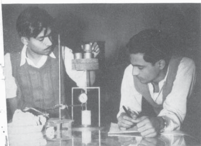
UNCONFINED COMPRESSION TEST EQUIPMENT
